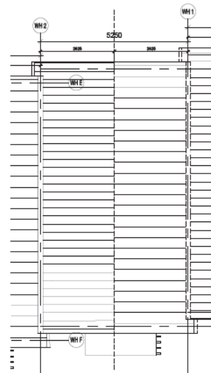
Typical mid terrace WH 2-7 ROOF PLAN
