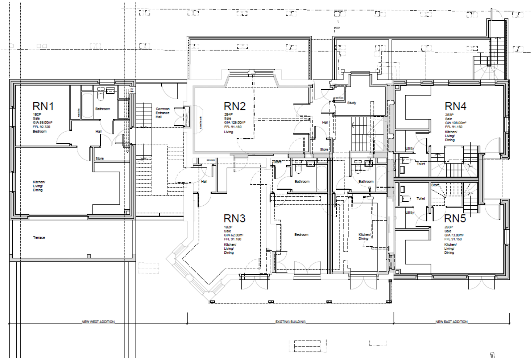
Roseneath First Floor Plan
